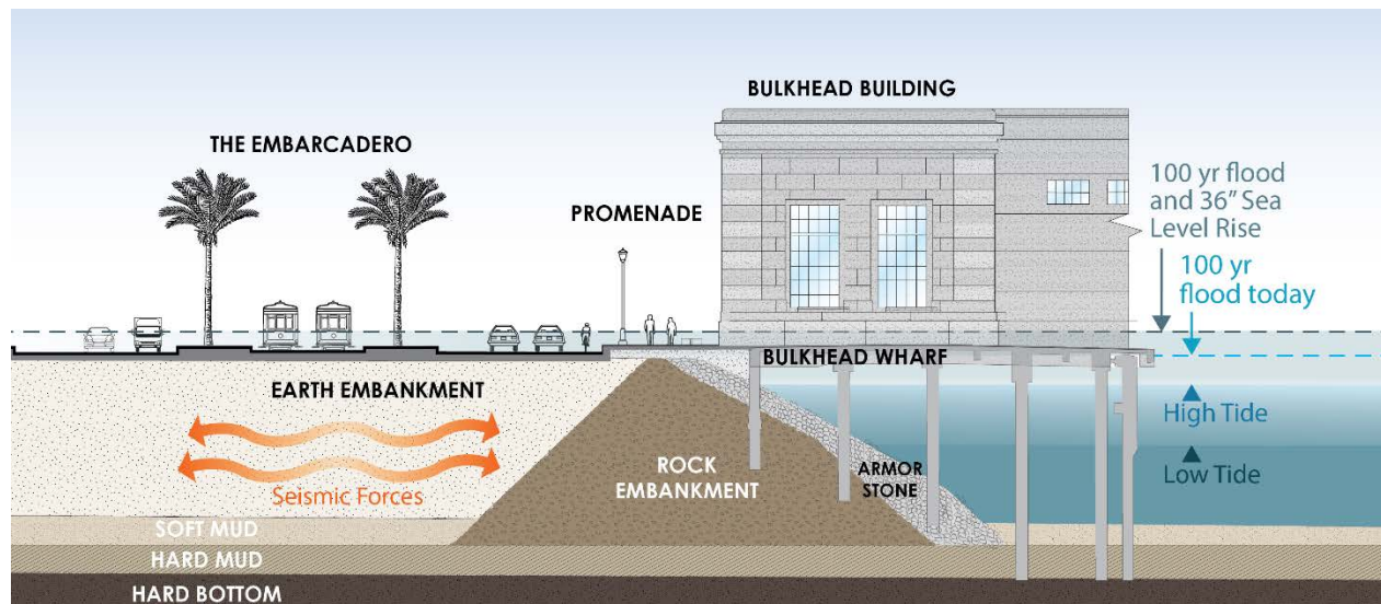
Figure 2: Seismic Risk to the Seawall
