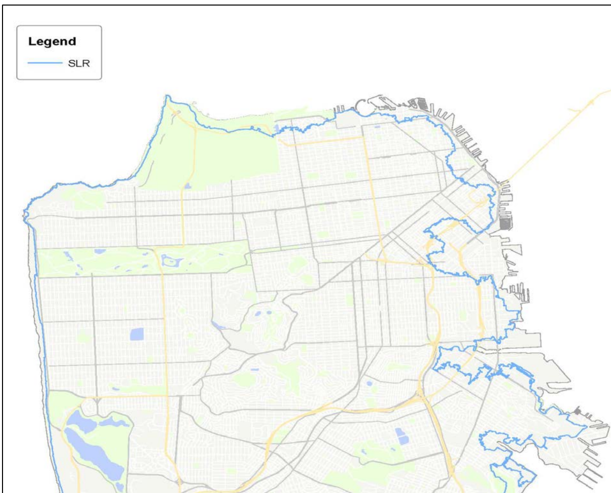
Figure 3: Sea Level Rise Vulnerability Zone Map
